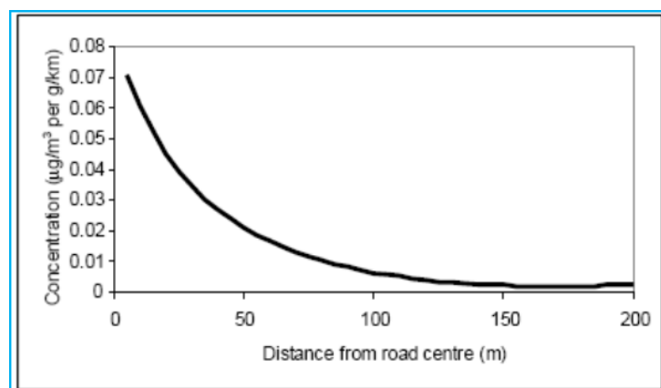
Figure 1: Example of traffic contribution to concentrations of pollutants at different distances from a road
