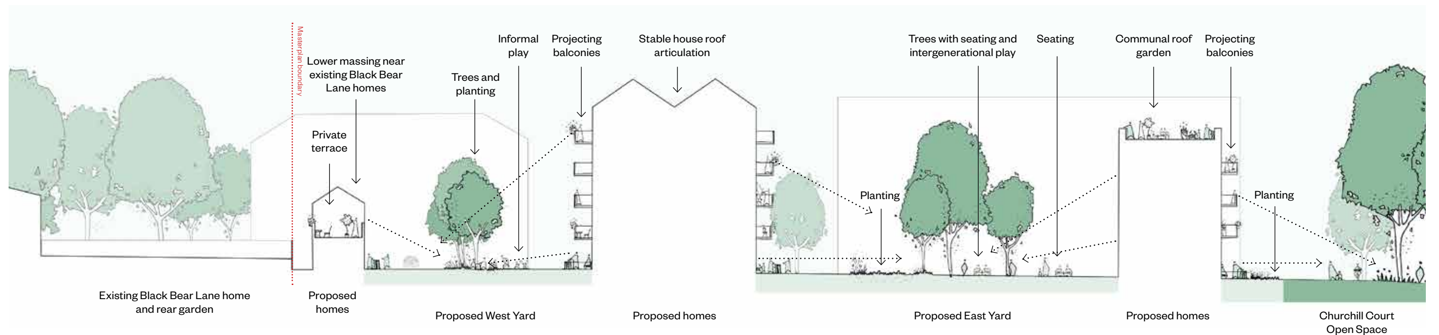
Fig.171 Section B through Churchill Yard courtyards, Black Bear Lane homes and Churchill Court Open Space
