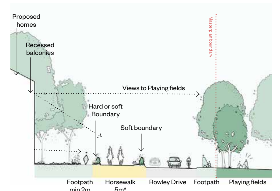
Fig.100 Rowley Drive Section B through Churchill Yards and playing fields
