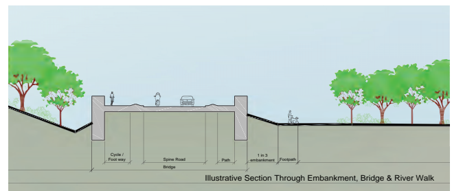
Illustrative section through spine road in river corridor area
