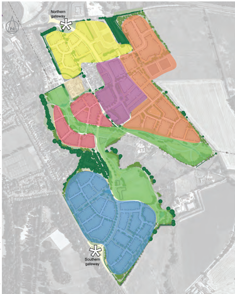
Figure 5.3 –Character areas
