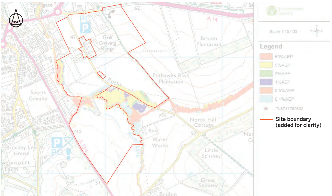
Figure 2.3 – Environment Agency Updated Flood Risk model (May 2015)
