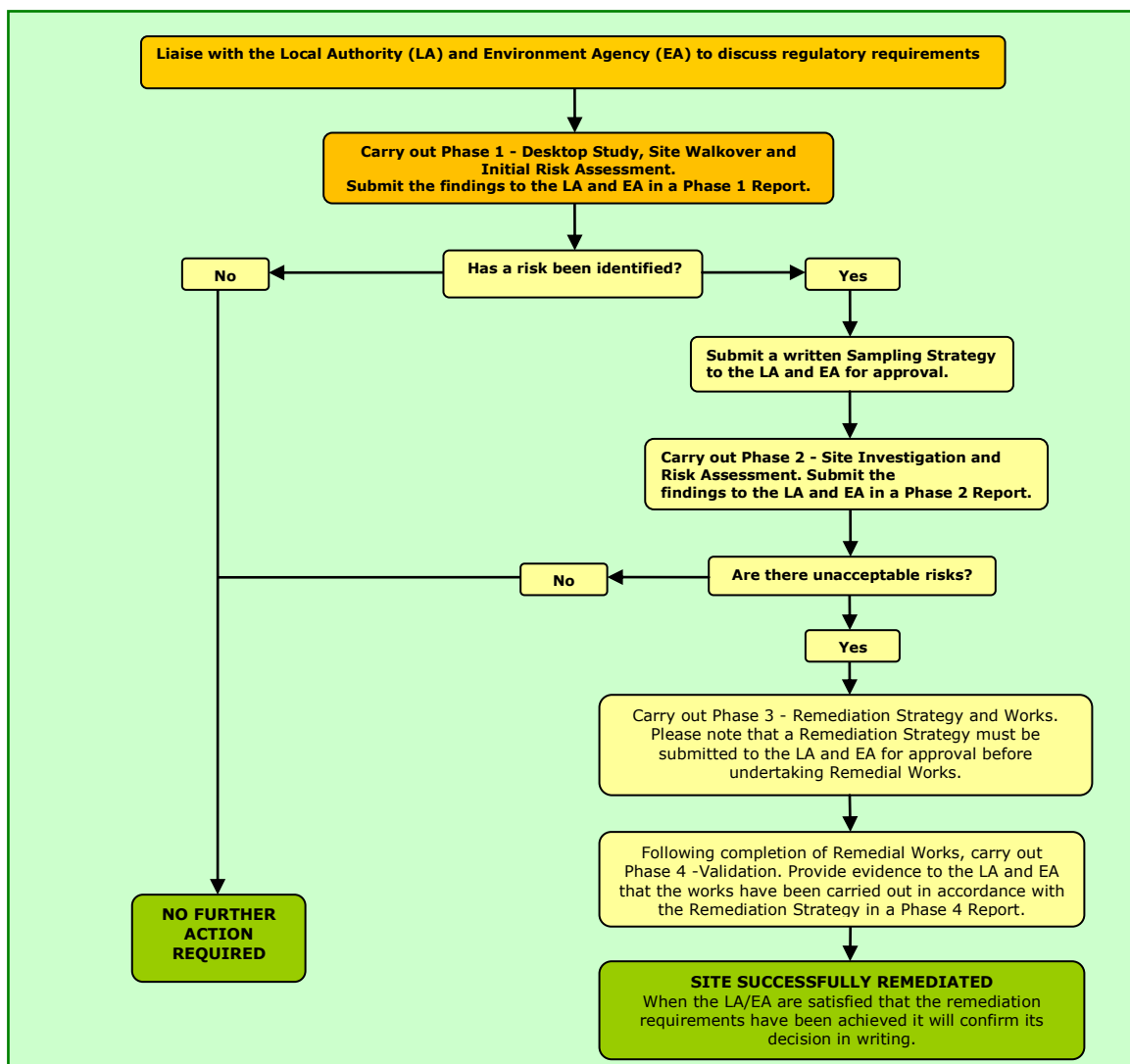
Figure 1. The investigation, assessment and remediation of land contamination
